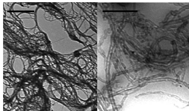
Fig. 1. TEM images of single- (left) and multi-walled (right) carbon nanotubes. While SWNT are present as bundles of different diameter and length, due to their strong aggregation tendency, MWNT can be instead observed as isolated entities. The scale bars correspond to 1 \mu\text{m} and 250 nm, respectively.
